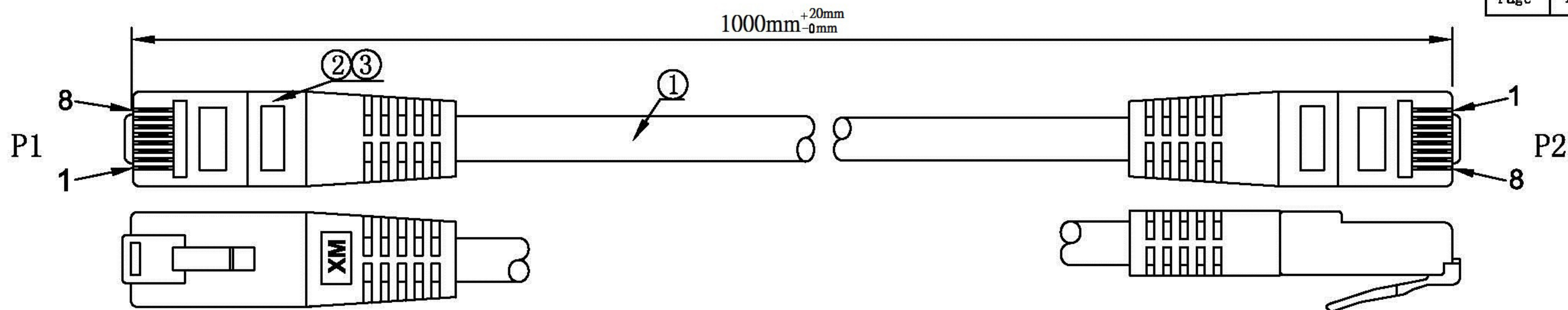
WIRING DIAGRAM
